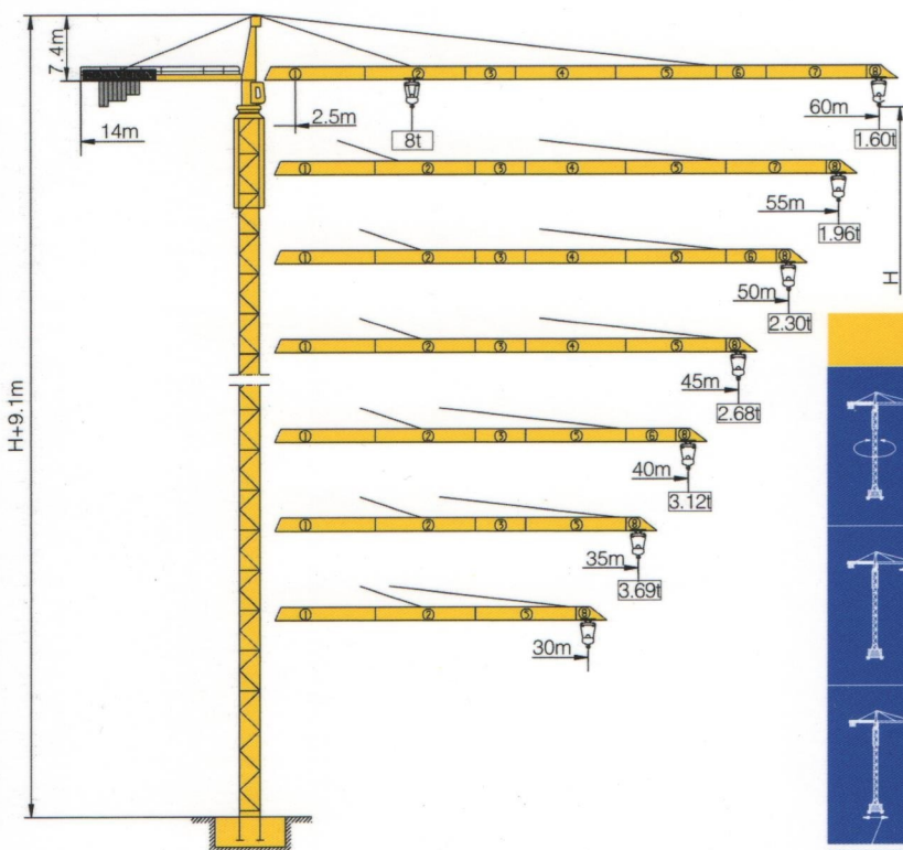
Load Diagrams
