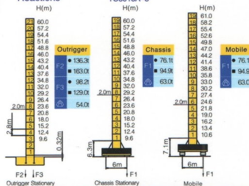
Masts Reactions
